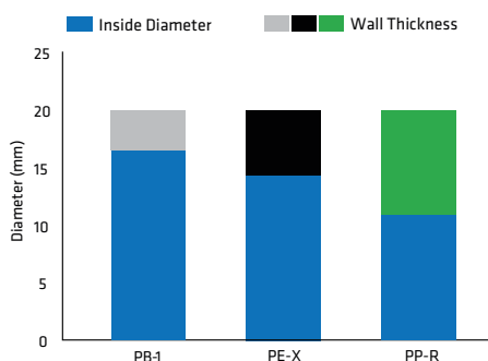
Different material thickness (service life class 2 ISO 10508)
