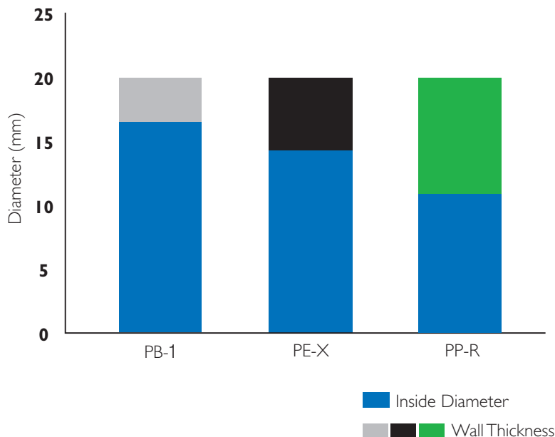
Different material thickness (service life class 2 ISO 10508)
