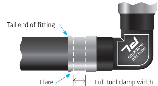
Correct Appearance Of Best Joint
